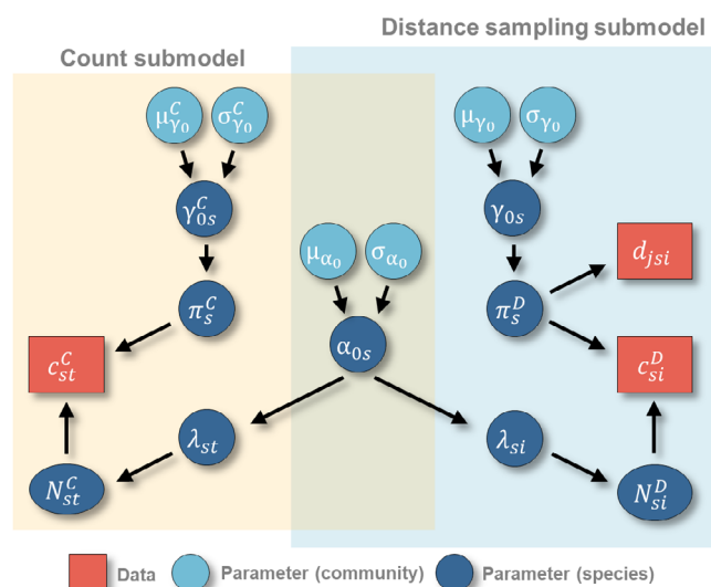
FIGURE 1 Graphical overview of integrated community model that combines distance sampling and count data. The parameters within the overlapping rectangles are shared between data sources. d_{jsi} is the distance measurements to animals from the distance sampling surveys. c_{st}^C and c_{sl}^D are the number of animals observed from the single-visit counts and distance sampling data, respectively, while N_{st}^C and N_{sl}^D are the corresponding latent abundances and \lambda_{st} and \lambda_{sl} the corresponding expected abundances. \alpha_{0s} is the species-level intercept for expected abundance and is modeled from a community distribution with mean \mu_{\alpha_0} and SD \sigma_{\alpha_0} . \pi_s^C and \pi_s^D are transect-level detection probabilities for the count and distance-sampling data, respectively, and are modeled via detection functions that include scale parameter intercepts \gamma_{0s}^C (counts) and \gamma_{0s}^D (distance sampling). These species-level intercepts are drawn from community-level distributions with means \mu_{\gamma_0}^C (counts) and \mu_{\gamma_0}^D (distance sampling) and SDs \sigma_{\gamma_0}^C (counts) and \sigma_{\gamma_0}^D (distance sampling). An updated graphical overview of the model for the case study is provided in Appendix S1: Figure S5.
