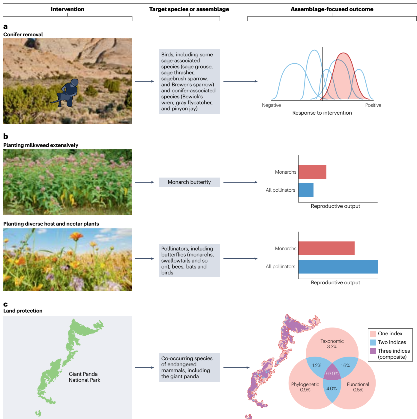
Fig. 2 | Examples of conservation interventions that can improve outcomes at the assemblage level. a, Targeted removal of conifers in sagebrush ecosystems benefits sagebrush-associated bird species but can harm conifer-associated bird species. Prioritizing sites for conifer removal based on predicted average responses in the sagebrush-associated bird assemblage led to overall positive responses 62 . b, Planting diverse plants in gardens can benefit the monarch butterfly, a species of substantial conservation concern, while also supporting the wider assemblage of pollinators. Planting only milkweed, the
